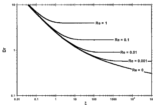
Figure 6. Effect of filament drawdown on aerodynamic drag.
