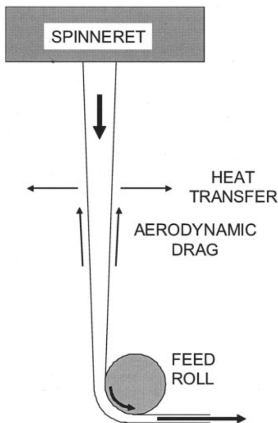
Figure 1. Fiber spinning operation.
